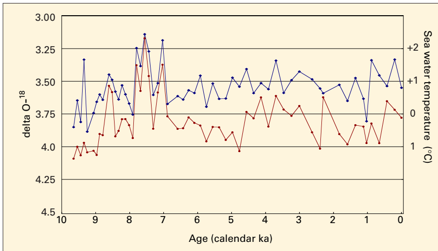
Figure 1: Local \delta^{18}\text{O} changes versus age in the planktonic species Neogloboquadrina pachyderma left coiling and the benthic species Elphidium clavatum in core ASV 880 (79°55'5 N, 47°08'2 E, water depth 388 m). The approximate temperature scale has been established assuming that the core top reflects modern conditions and that the water temperature decreases by 1°C when the foraminifer \delta^{18}\text{O} value increases by 0.25‰ [Reference: Duplessy et al. (in press) Holocene paleoceanography of the Northern Barents Sea and variations of the northward heat transport by the Atlantic Ocean, Boreas. ]
