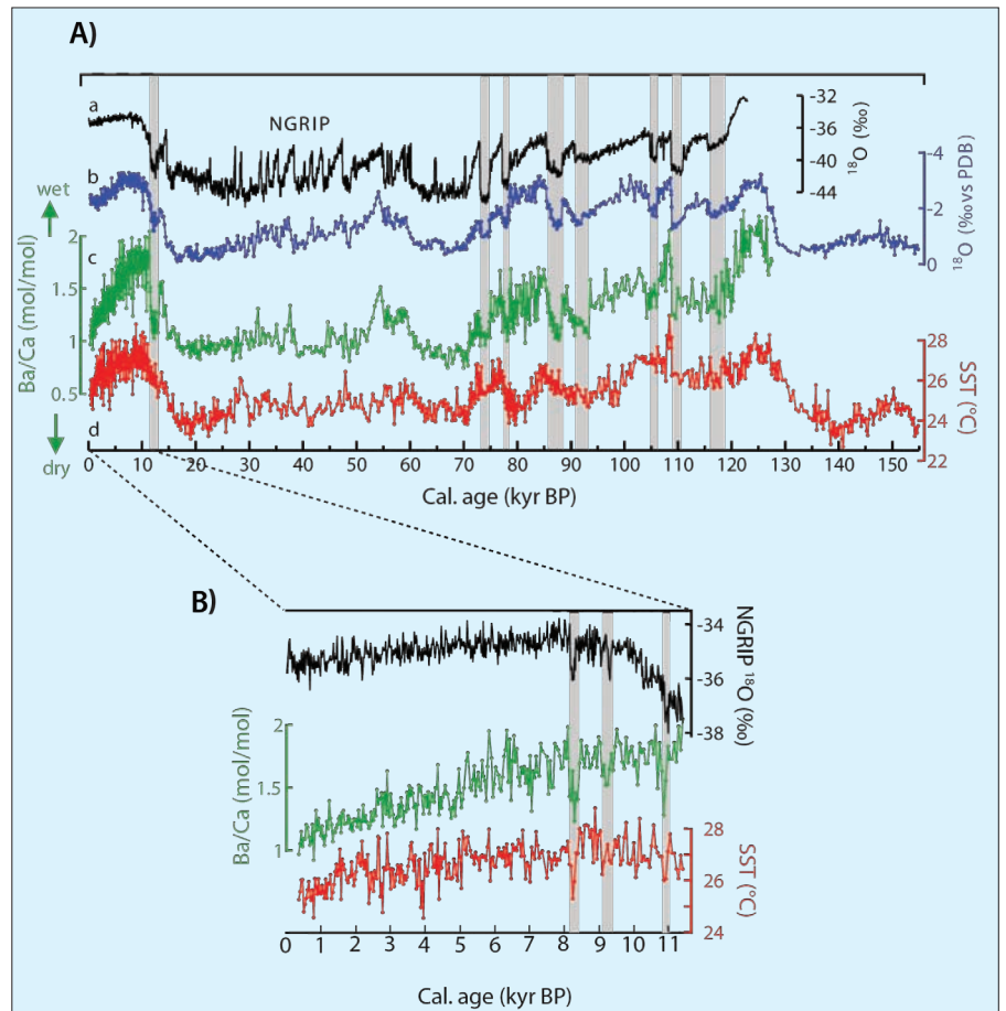
Figure 2: A) Proxy records from shallow-dwelling planktic foraminifers ( Globigerinoides ruber , pink variety) of core MD03-2707 (b-d) compared (a) with isotope composition of Greenland ice core (NGRIP members, 2004). (b) oxygen isotope composition, (c) Ba/Ca used as indicator of changes in riverine runoff, and (d) Mg/Ca-based SST estimate. Gray bars indicate intervals of relatively weak monsoon precipitation that tightly correlate with cold events in the Greenland ice core record (NGRIP). B) Enlarged section covering the past 11.5 kyr BP. Gray bars indicate periods of low monsoon precipitation that coincide or overlap with cold air temperature over the northern high latitudes and fresh water discharges into the North Atlantic Ocean (e.g., Clark et al., 2001).
