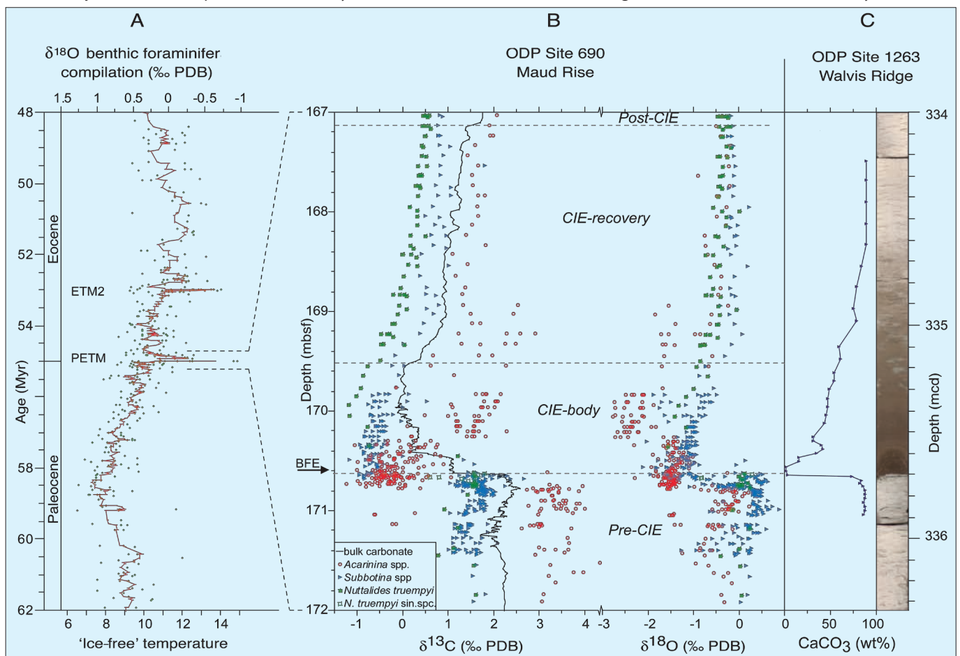
Figure 1: A ) Benthic foraminifer \delta^{18}\text{O} record from 62–48 Myr (adapted from Zachos et al., 2001; data for ETM2 represent the Cibicidoides record from Lourens et al., 2005). \delta^{18}\text{O} values represent corrected values (cf. Zachos et al., 2001). An additional correction of -0.25\text{‰} was applied to the ETM2 Cibicidoides values to synchronize baseline levels between the records. ETM2 = Eocene Thermal Maximum 2 (also referred to as H1 or Elmo), PETM = Paleocene-Eocene Thermal Maximum. B ) Compilation of \delta^{13}\text{C} and \delta^{18}\text{O} values across the PETM of planktic foraminifers (surface dweller Acarinina and thermocline dweller Subbotina spp.; mostly single specimens), benthic foraminifer ( Nuttallides truempyi ) and bulk carbonate from ODP Site 690 from Maud Rise in the Weddell Sea (data compilation and figure modified from Sluijs et al., 2007a). C ) Carbonate weight % record and core photo of ODP Site 1263 at Walvis Ridge, southeastern Atlantic (adapted from Zachos et al., 2005), showing dissolution and resulting clay layer. BFE refers to the main phase of benthic foraminifer extinction, mbsf = meters below sea floor; mcd = meters composite depth.
