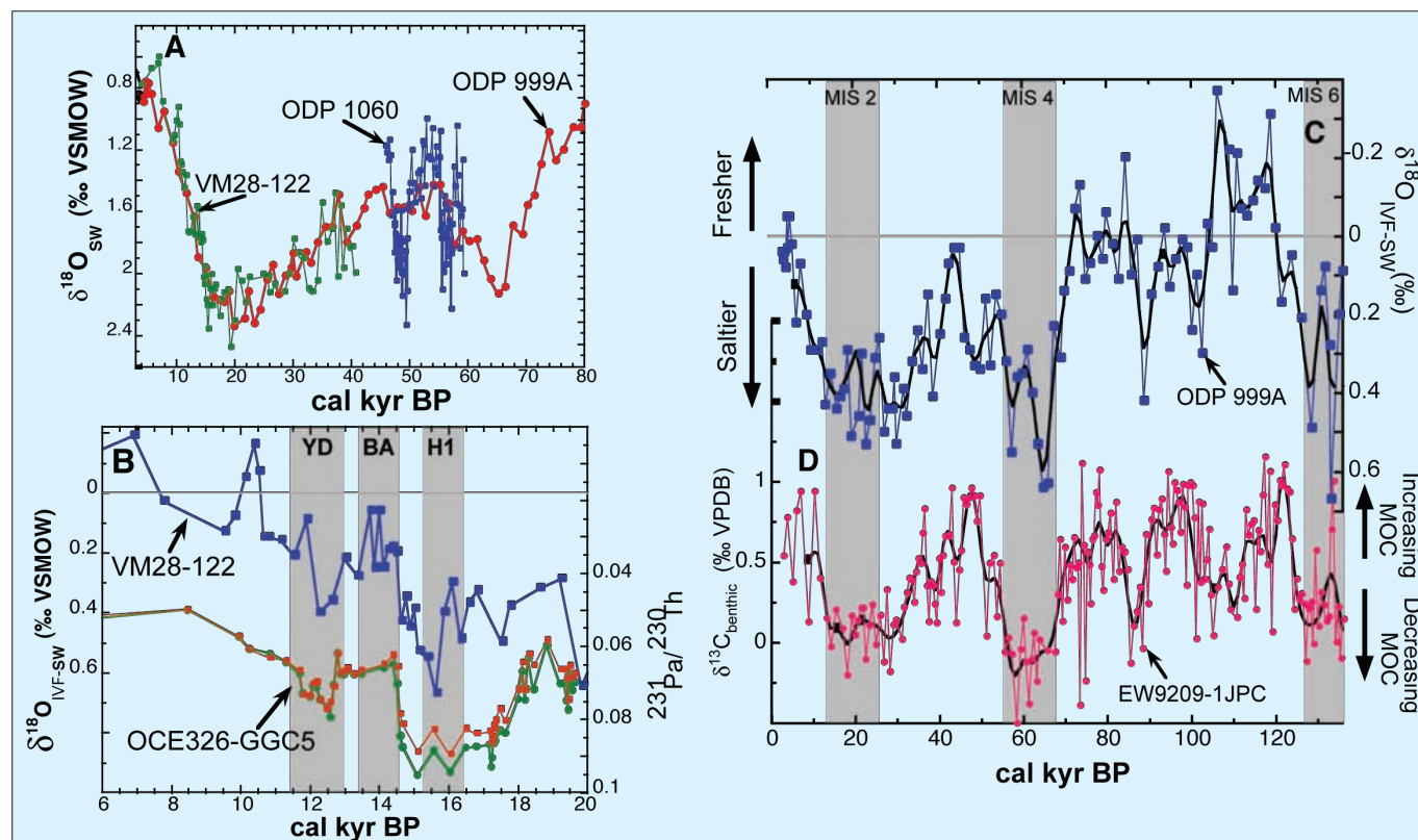
Figure 2: A ) Computed \delta^{18}\text{O}_{sw} records from the Caribbean at sites ODP 999A (red line) and VM28-122 (green line) and in the North Atlantic gyre at ODP 1060 (blue line) during the last glacial cycle. \delta^{18}\text{O}_{sw} values calculated from Mg/Ca-derived SST and \delta^{18}\text{O}_c in planktic foraminifer G. ruber . To compare regional \delta^{18}\text{O}_{sw} change between Caribbean and gyre site 1060, modern \delta^{18}\text{O}_{sw} difference between the two sites (0.3‰) was subtracted from ODP 1060 values to account for additional evaporation that occurs as waters transit between the tropics and subtropics. After removing global \delta^{18}\text{O}_{sw} change due to continental ice volume (Waelbroeck et al., 2002), local \delta^{18}\text{O}_{sw} records were normalized to modern regional value, resulting in ice volume free \Delta\delta^{18}\text{O}_{IVF-SW} record from VM28-122 ( B ; blue line) and 999A ( C ; blue line) during the last glacial cycle. Note the rapid salinity decrease recorded in the Caribbean at VM28-122 at 14.6 cal kyr BP corresponds to a decrease in ^{231}\text{Pa}/^{230}\text{Th} ratios in Bermuda Rise core OCE 326-GGC5 ( B ; red line) (McManus et al., 2004), indicating a strengthening of AMOC at the beginning of BA. Shaded bars also illustrate Heinrich Event 1 (H1) and Younger Dryas (YD). C ) \Delta\delta^{18}\text{O}_{IVF-SW} from ODP 999A (black line is a low-pass (5 kyr) filter with 5-point filter weight running through raw data (blue line)). Benthic \delta^{13}\text{C} record ( D ) (black line is a low-pass (5 kyr) filter with 10-point filter weight) from Ceara Rise core EW9209-1JPC (5°N, 43°W; 4,056 m; pink line) indicates times of reduced AMOC (lower \delta^{13}\text{C} ) (Curry and Oppo, 1997) when \Delta\delta^{18}\text{O}_{IVF-SW} in ODP 999A are enriched.
