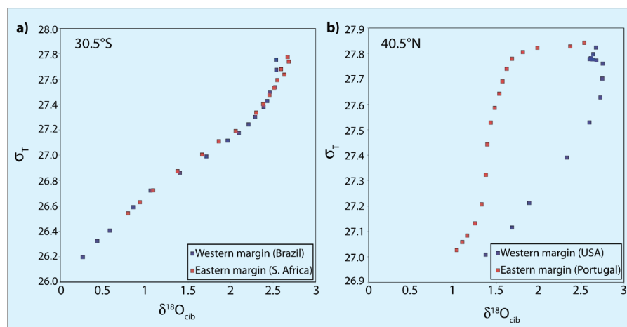
Figure 2: a) Relationship between seawater density ( \sigma_t ) and calculated \delta^{18}\text{O} of benthic foraminifers calcifying in this water on the eastern and western margins of the South Atlantic between 200–2000 m water depth. Note that water mass properties are relatively similar on either side of the basin; b) Relationship between seawater density ( \sigma_t ) and \delta^{18}\text{O} of benthic foraminifers on eastern and western margins of the North Atlantic between 200–2000 m water depth. The input of Mediterranean Outflow Water (MOW) just south of this section produces dissimilar water mass properties on either side of the North Atlantic at 40°N. While the impact of the MOW will be less at higher or lower latitudes, the relationship between \delta^{18}\text{O} of foraminifers and water density ( \sigma_t ) must be determined on each margin using independent reconstructions of temperature and salinity.
