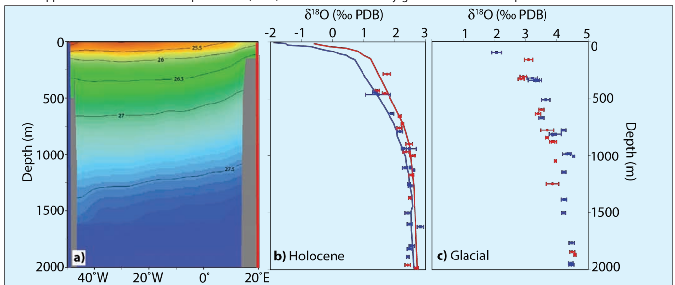
Figure 1: a ) Seawater density ( \sigma_t ) along a zonal section at 30°S in the Atlantic (Conkright et al., 2002). The east-west density contrast reflects the shear in the meridional overturning circulation at this latitude; b ) Oxygen isotopic composition ( \delta^{18}\text{O} ) of benthic foraminifers in recent sediments on the eastern (red symbols, mean and standard deviation for each core) and western (blue symbols) sides of the basin reflects the density contrast across the basin. Solid lines are predicted \delta^{18}\text{O} based on modern hydrographic data (modified from Lynch-Stieglitz et al., 2006); c ) Oxygen isotopic composition of benthic foraminifers from the Last Glacial Maximum suggest that the modern density contrast in the upper 2 km was absent or reversed (modified from Lynch-Stieglitz et al., 2006).
