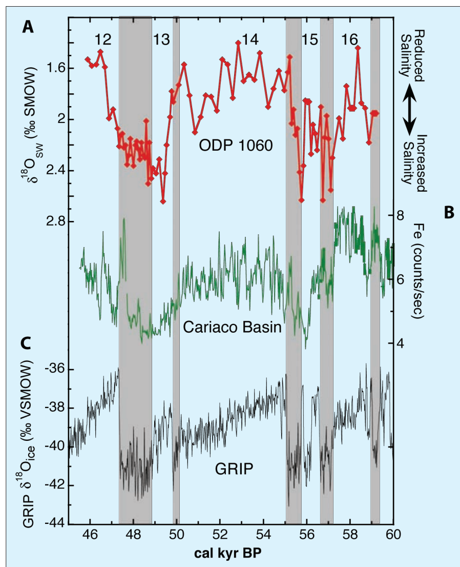
Figure 3: Salinity variation at ODP site 1060 during MIS 3. A ) Computed \delta^{18}\text{O}_{\text{SW}} from site 1060; B ) Fe content (counts/sec) from Cariaco Basin core ODP 1002 (Peterson et al., 2000), adjusted to the GRIP age model; C ) GRIP \delta^{18}\text{O}_{\text{ICE}} record (Johnsen et al., 2001). Cold stadials in the GRIP record are marked by more arid conditions in the western tropical Atlantic (lower Fe concentrations) and elevated gyre salinities (increased \delta^{18}\text{O}_{\text{SW}} values at site 1060). Note the salinity increases (as \delta^{18}\text{O}_{\text{SW}} ) associated with the shaded stadial events and the reduced salinities associated with the numbered interstadials 12-16.
