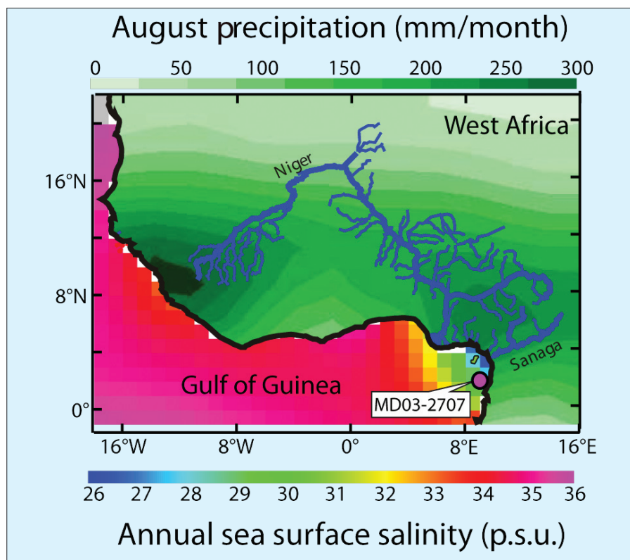
Figure 1: Location of MD03-2707, drainage basin of the Niger and Sanaga Rivers, precipitation in August (the height of West African monsoon precipitation) (Janowiak and Xie, 1999), and annual sea surface salinity in the Gulf of Guinea (Levitus and Boyer, 1994). Note: the drainage basins of the Niger and Sanaga Rivers cover a large part of the West African monsoon, and riverine runoff heavily affects the hydrography over the core site (Weldeab et al., 2007b).
