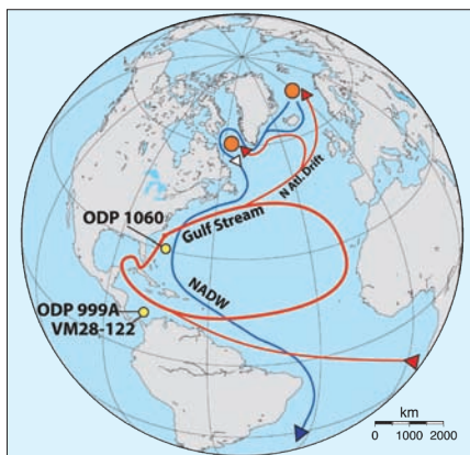
Figure 1: Modern N. Atlantic surface (red) and deep water (blue) circulation and location of Caribbean cores ODP 999A (12°45'N, 78°44'W; 2,827 m; 4 cm/kyr sed. rate) and VM28-122 (11.56°N, 78.41°W; 3,623 m; 4-15 cm/kyr sed. rate) and N. Atlantic subtropical gyre core ODP 1060 (30°46'N, 74°28'W; 3480 m; 20-53 cm/kyr sed. rate). Orange circles indicate sites of deepwater formation in N. Atlantic.
