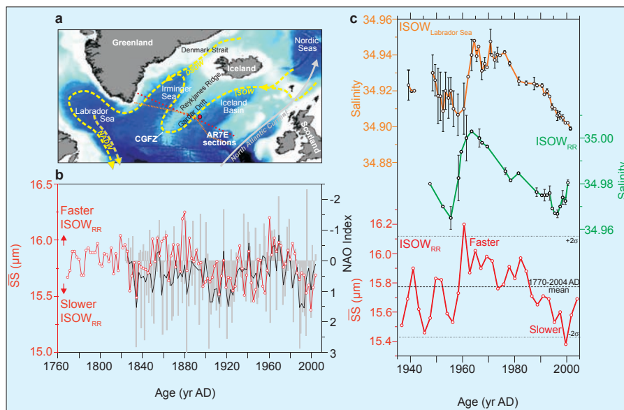
Figure 1: a ) Map of North Atlantic Ocean with schematic pathway of ISOW (yellow line), DSOW (yellow line), NADW (yellow line) and the North Atlantic Current (grey line). Location of RAPID-21-12B core indicated (red circle), and hydrographic sections (AR7E section) of Fig. 2 are shown for 1966 (red, dashed) and 1994 (orange, dotted). Location of Charlie Gibbs Fracture Zone (CGFZ) is also indicated; b ) Evidence of linear relationship between near-bottom flow-speed changes of ISOW on the eastern flank of Reykjanes Ridge ( ISOW_{RR} ) and NAO index: Sortable silt mean grain size ( \overline{SS} ) record of core RAPID-21-12B (red); winter NAO index (grey bars, reverse scale), 7-year smoothed NAO index (black); c ) Salinity time series of ISOW in Labrador Sea (orange) and eastern Reykjanes Ridge (green), \overline{SS} record of core RAPID-21-12B (red). Figure modified from Boessenkool et al., 2007.
