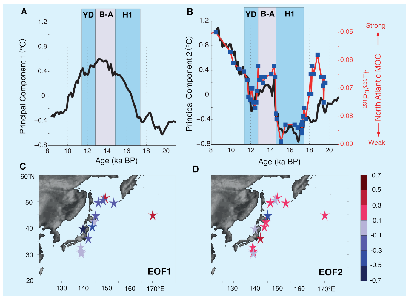
Figure 2: Empirical orthogonal function (EOF) analysis of alkenone-derived temperatures throughout 22-8 ka BP. A ) First principal component [°C] corresponding to EOF1 pattern. B ) Second principal component [°C] corresponding to the EOF2 pattern, along with estimates of North Atlantic meridional overturning circulation (McManus et al. 2004). C ) EOF1 and D ) EOF2 spatial patterns [unitless]. The color scale indicates the loading of the EOF pattern.
