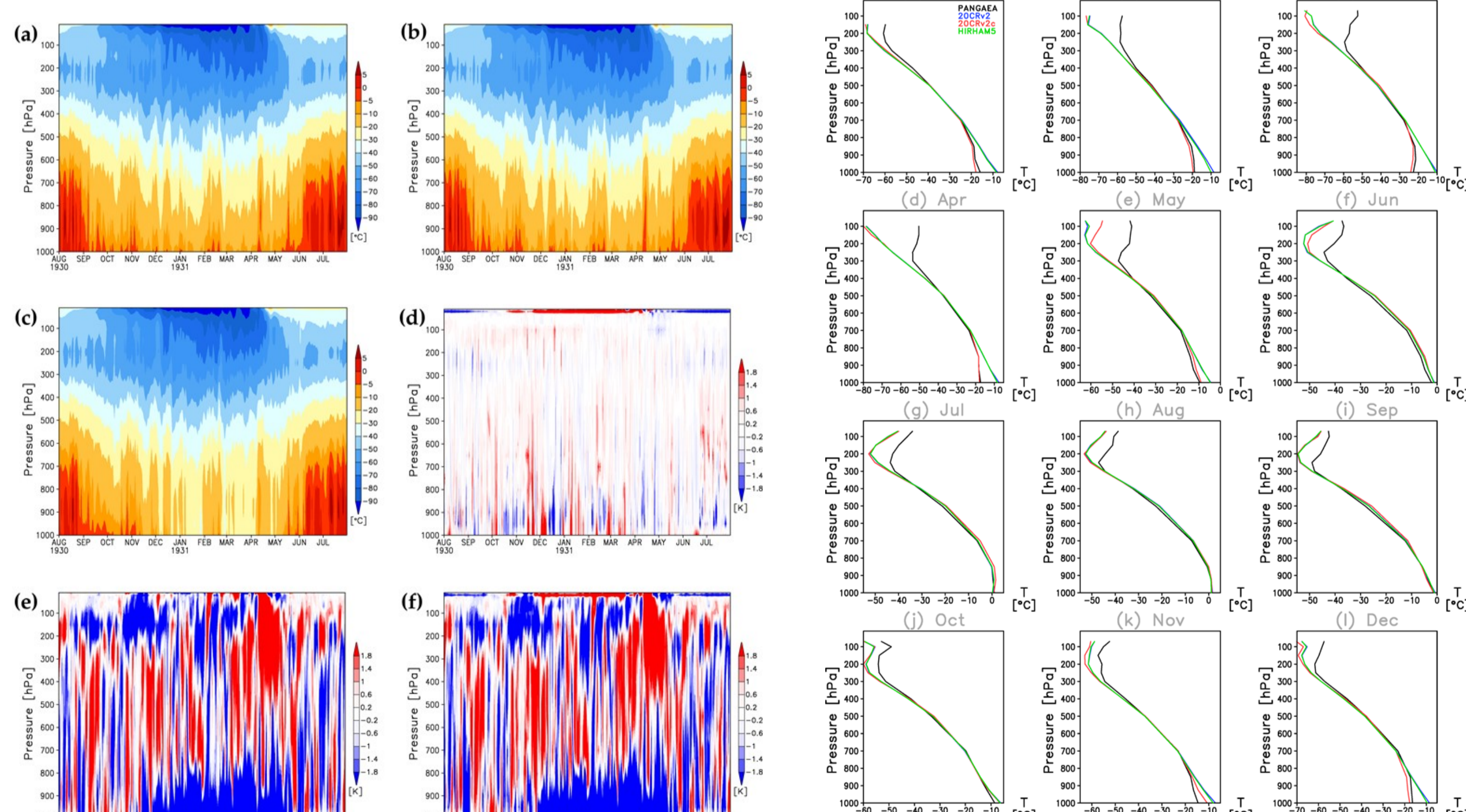
Multi-year (10 September 1934 - 31 December 1940) monthly temperature profiles for Calm Bay from PANGAEA observations (black), the newer (20CRv2c; red) and older (20CRv2; blue) version of 20CR, and the HIRHAM5 model (green). The calculation of monthly means always exploited the missing values from the daily PANGAEA data to take into account unavailable or vertically interrupted temperature profiles also in the reanalysis and model data. Temperatures are shown on the 16 standard pressure levels used by PANGAEA.
